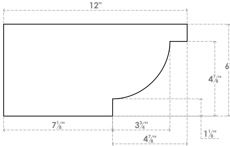
SIDE PROFILE
